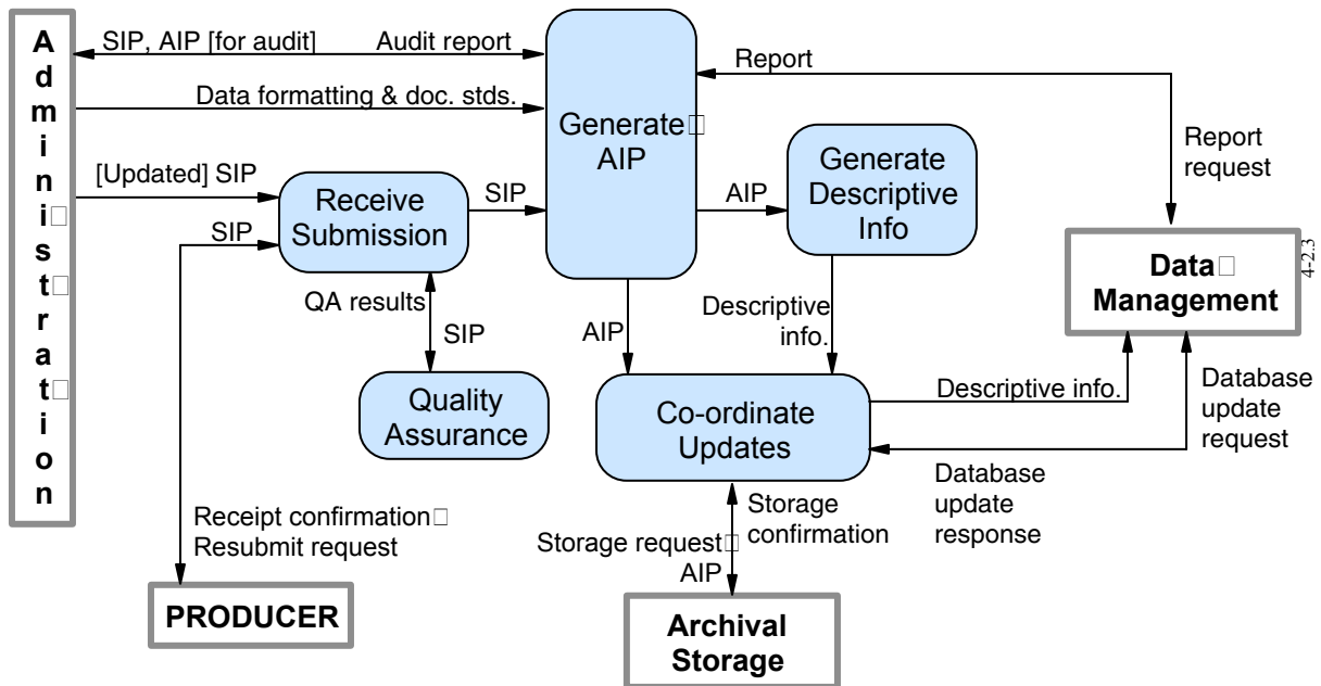
Figure 4-2: Functions of Ingest
