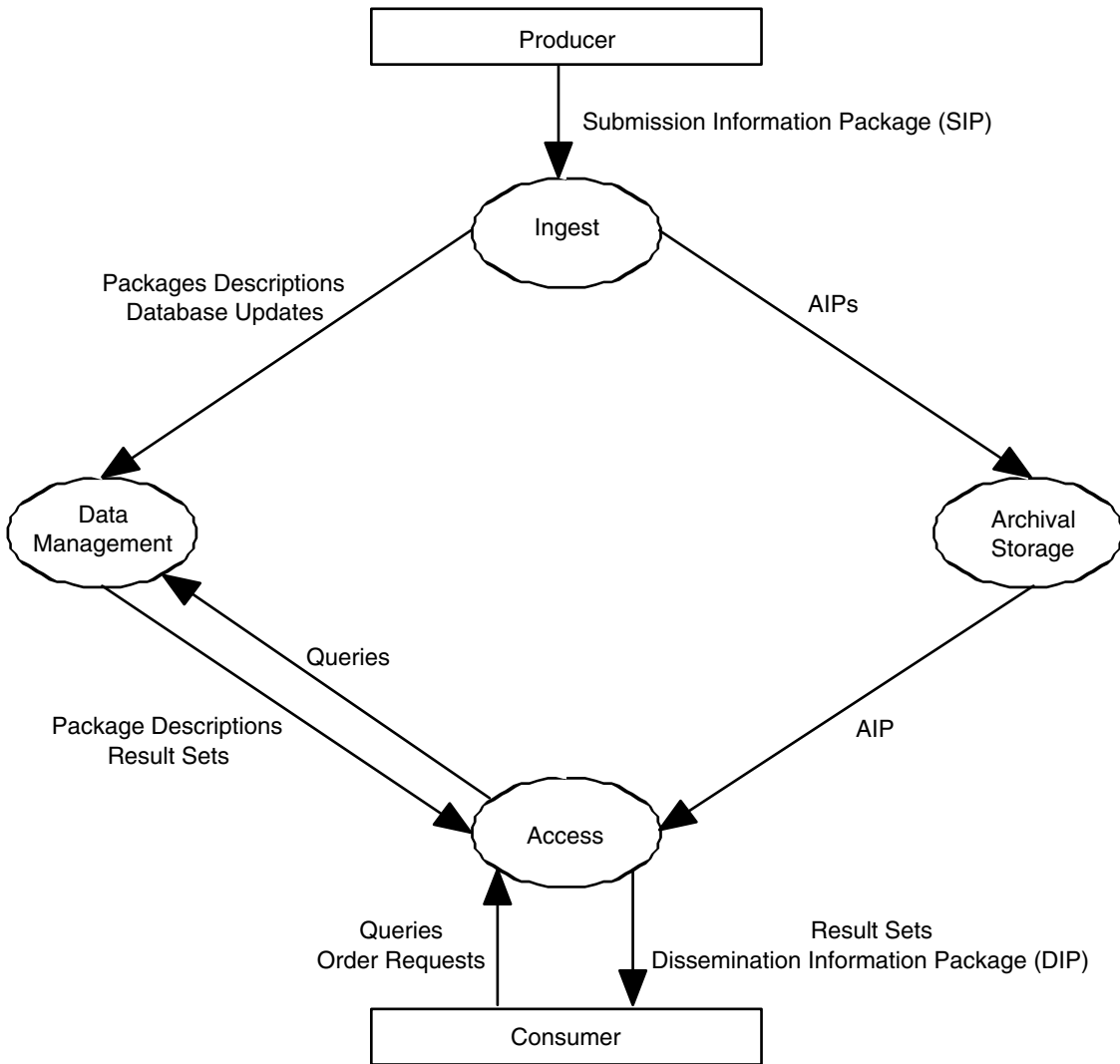
Figure 4-26: High-Level Data Flows in an OAIS
