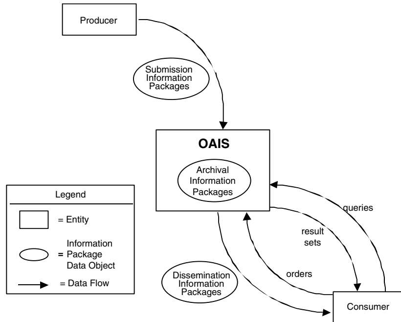
Figure 2-4: OAIS Archive External Data
