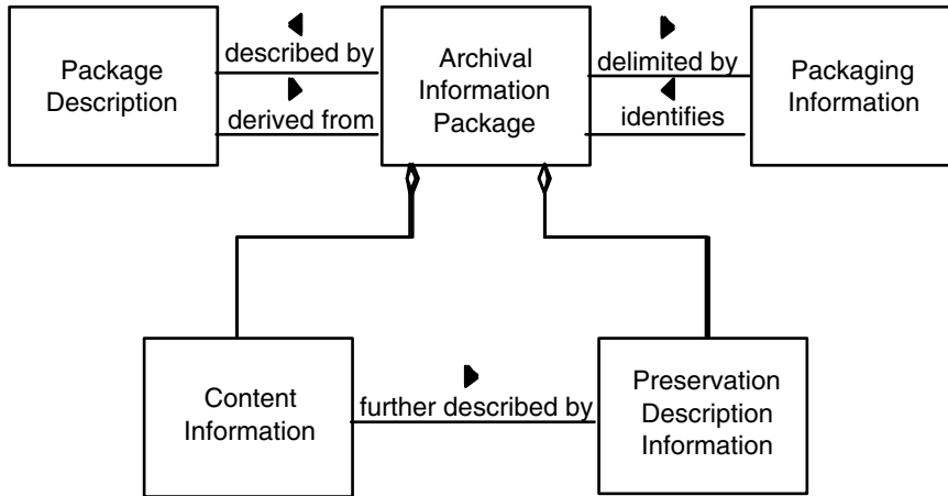
Figure 4-15: Archival Information Package (AIP)
