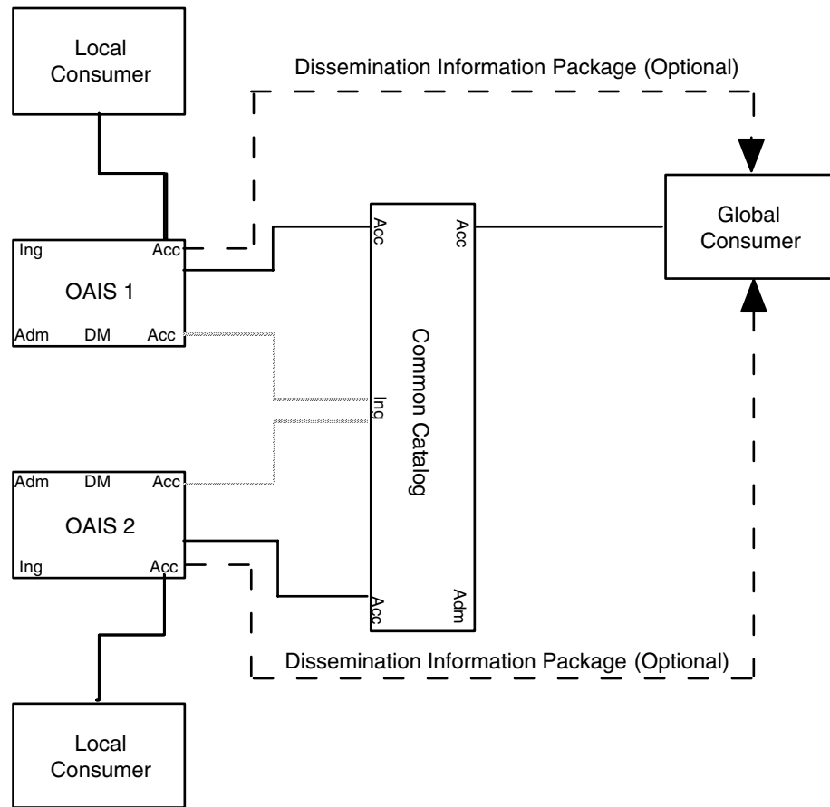
Figure 6-3: An OAIS Federation Employing a Common Catalog
